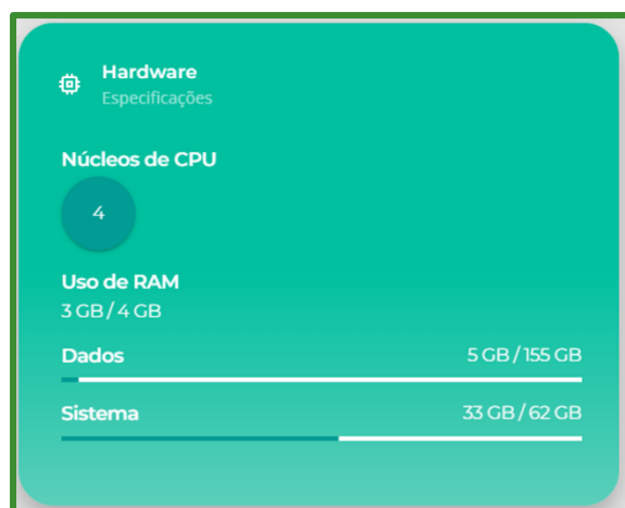
Figura 13: Painel - Hardware
